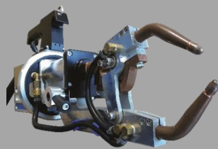
REF: STA10005 X-GUN ADAPTER c/w
